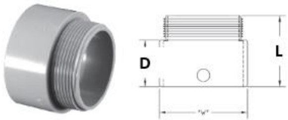
2" through 6" Terminal (Male) Adapter
