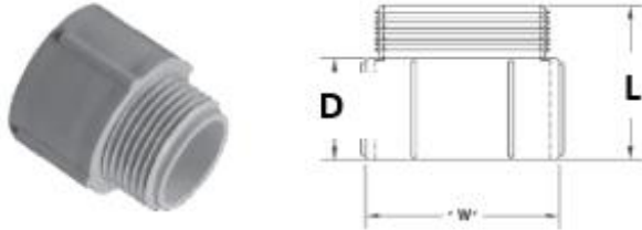
2" through 6" Terminal (Male) Adapter
